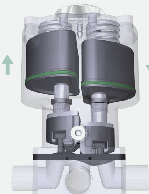
Valve 1 open / valve 2 closed
