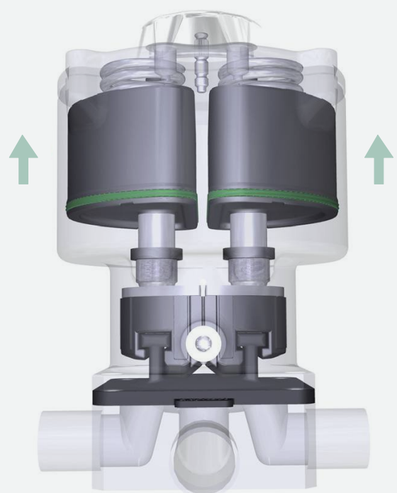
Valve 1 / valve 2 open
