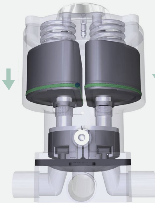
Valve 1 / valve 2 closed
