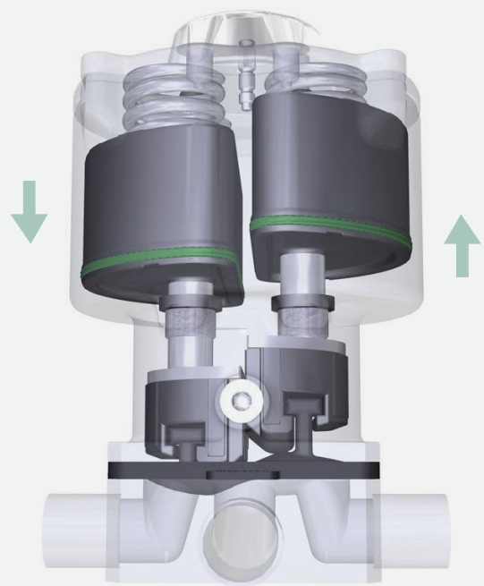
Valve 1 closed / valve 2 open
